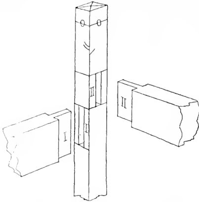
FIG. 239. MARKED DUPLICATE PARTS AND JOINTS.
